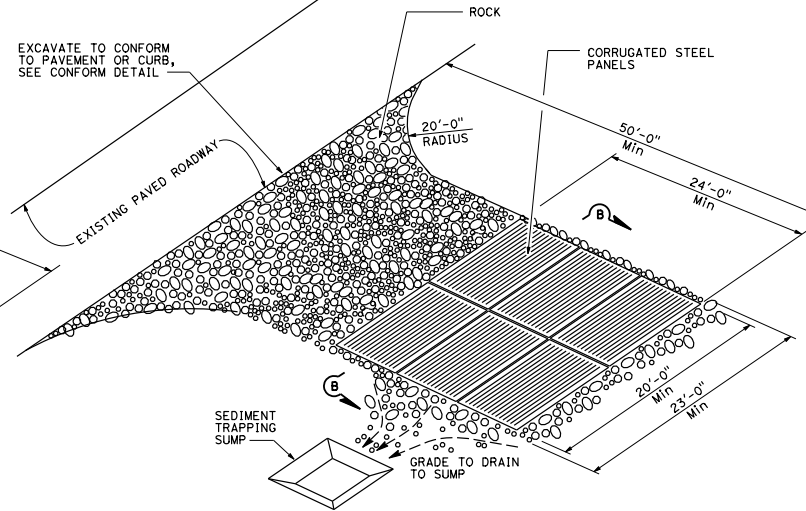
PERSPECTIVE TEMPORARY CONSTRUCTION ENTRANCE (TYPE 2)
