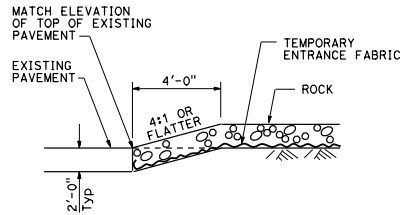
SECTION CONFORM DETAIL
